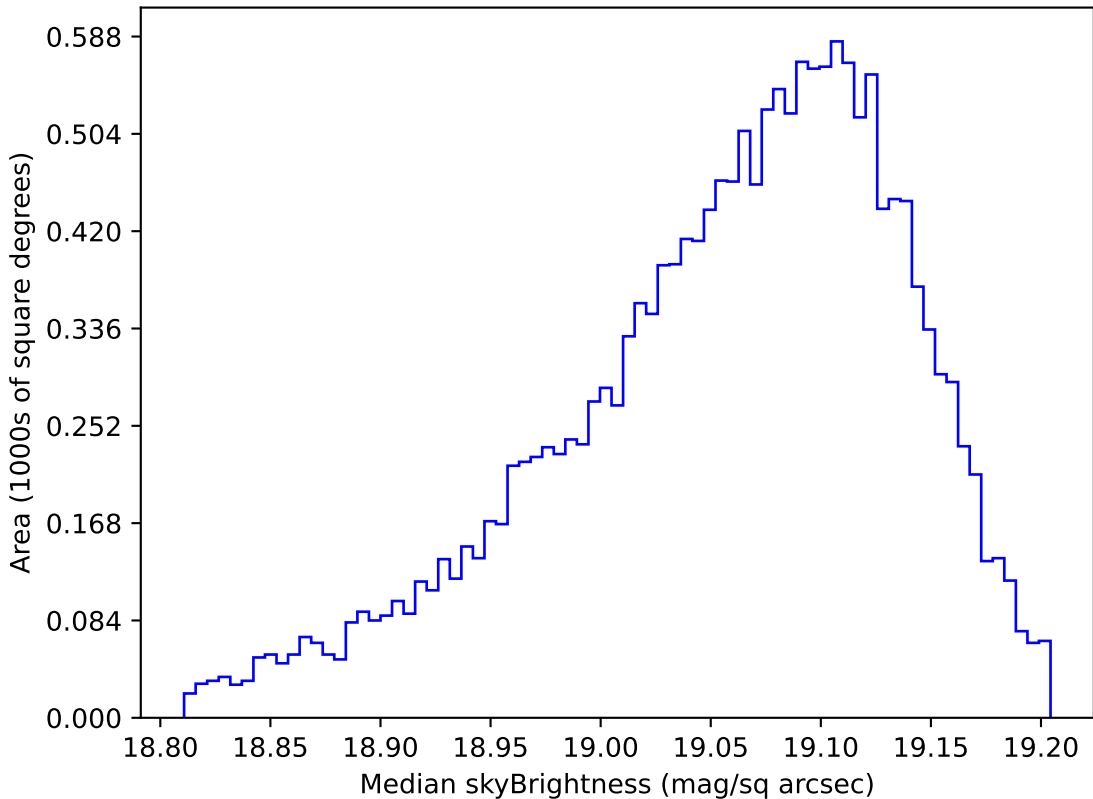
weather_cloudso31v3.4_10yrs WFD z band: Median skyBrightness
