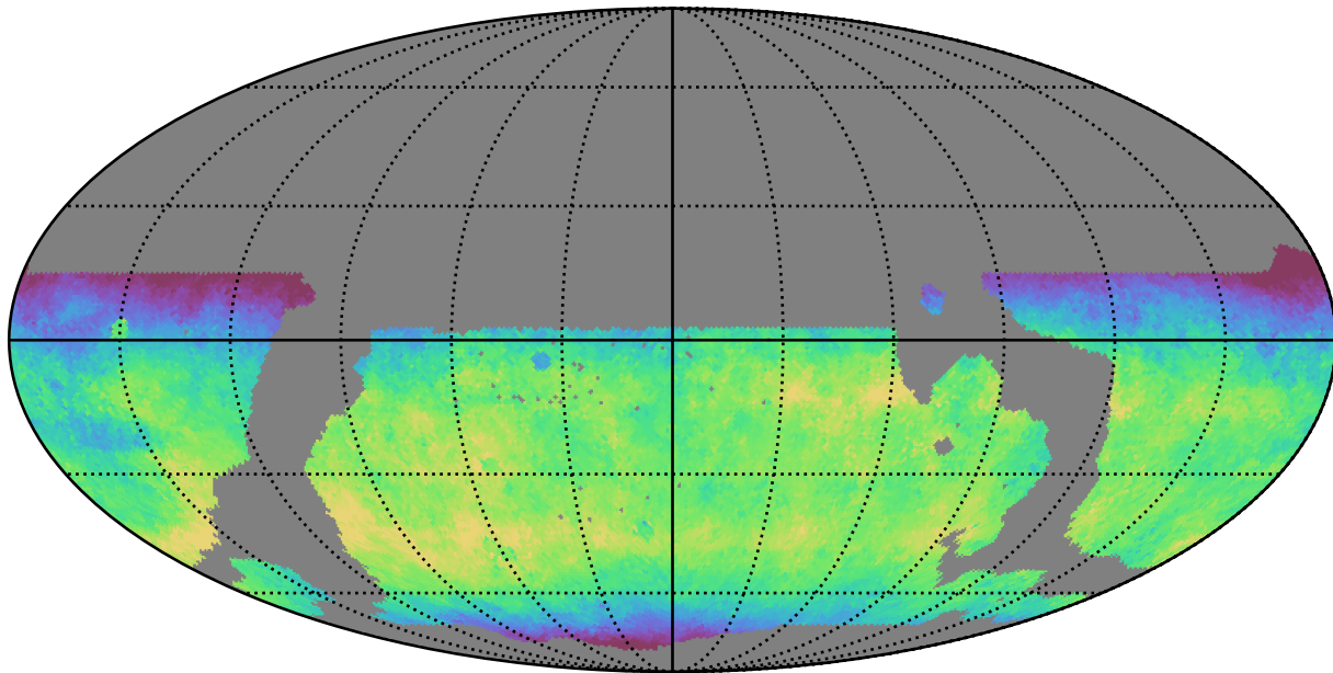
weather_cloudso31v3.4_10yrs WFD y band: Median skyBrightness
