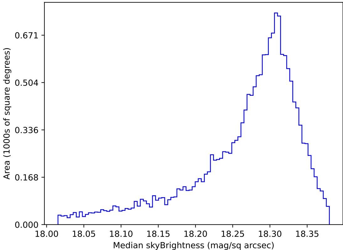
weather_cloudso31v3.4_10yrs WFD y band: Median skyBrightness
