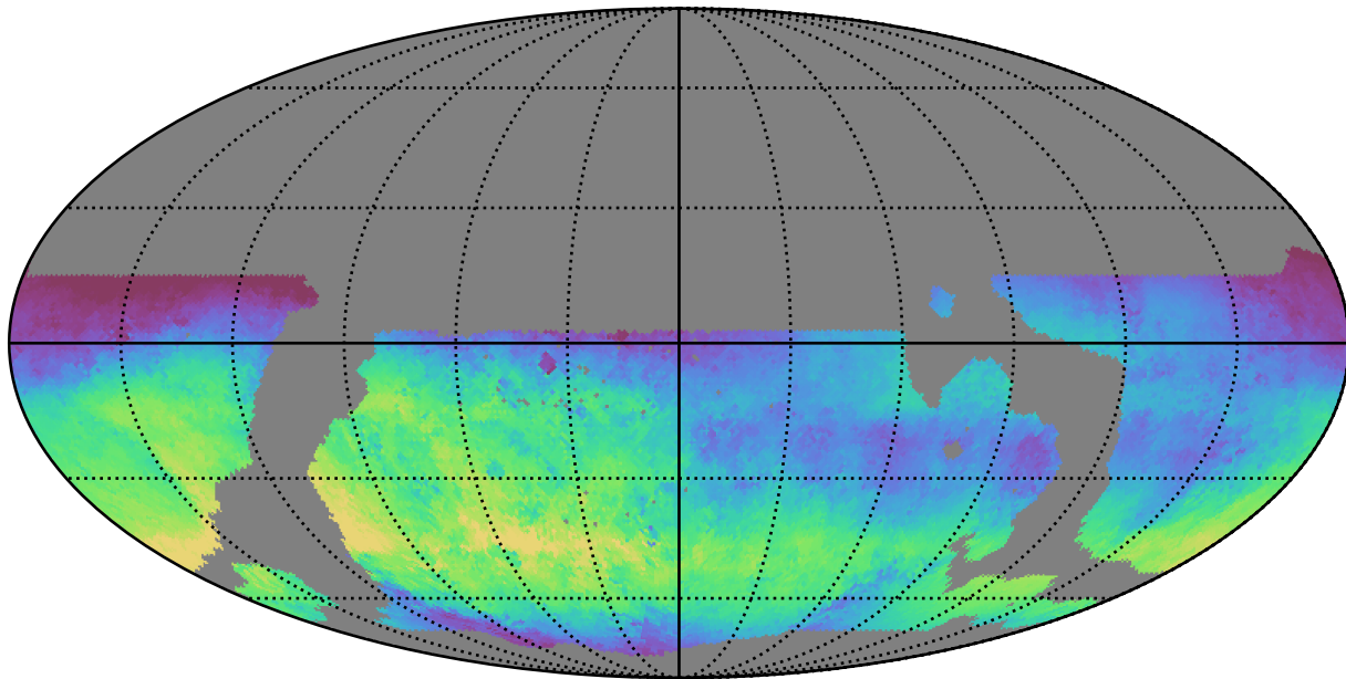
weather_cloudso31v3.4_10yrs WFD u band: Median skyBrightness
