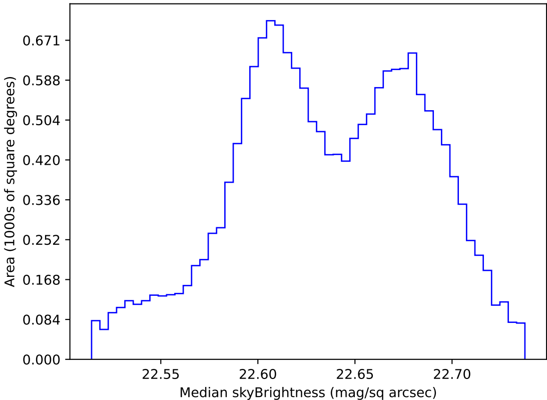
weather_cloudso31v3.4_10yrs WFD u band: Median skyBrightness
