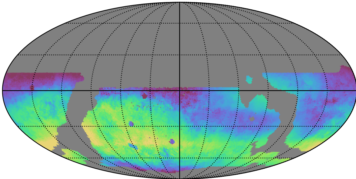
weather_cloudso31v3.4_10yrs WFD r band: Median skyBrightness
