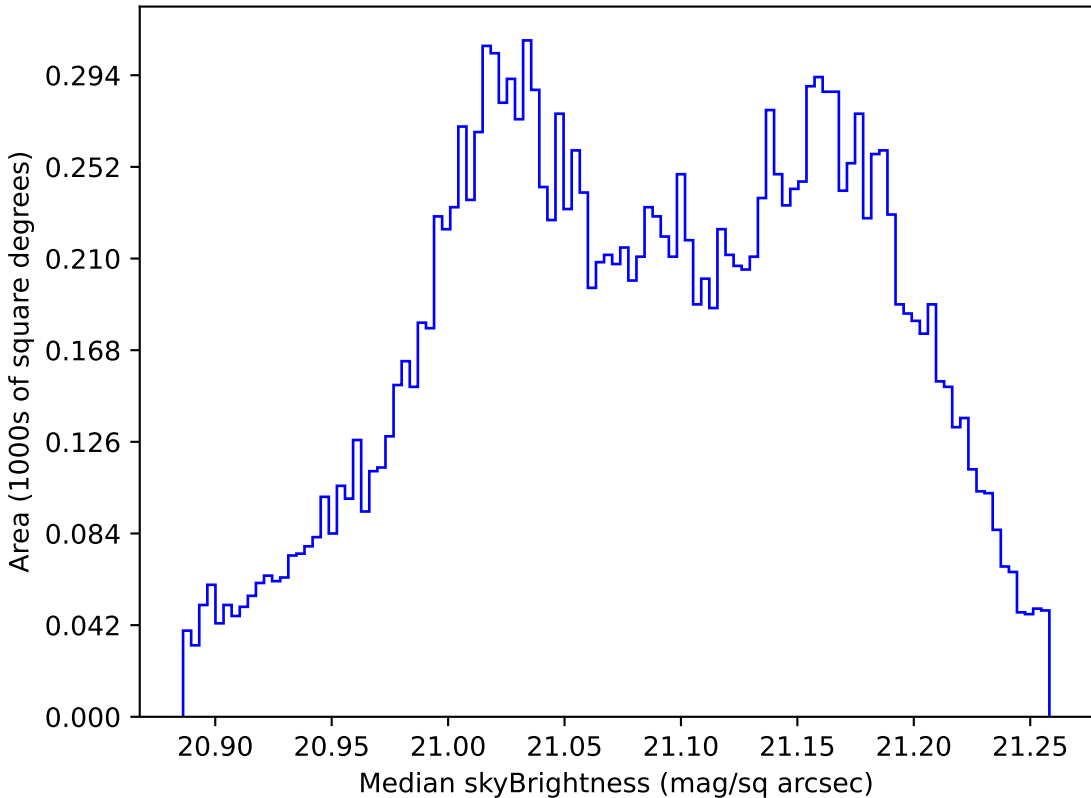
weather_cloudso31v3.4_10yrs WFD r band: Median skyBrightness
