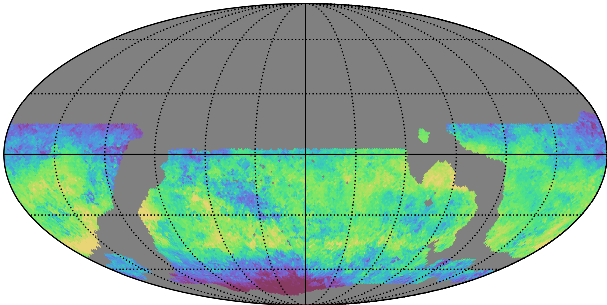
weather_cloudso31v3.4_10yrs WFD i band: Median skyBrightness
