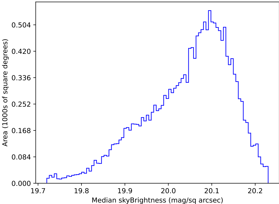
weather_cloudso31v3.4_10yrs WFD i band: Median skyBrightness
