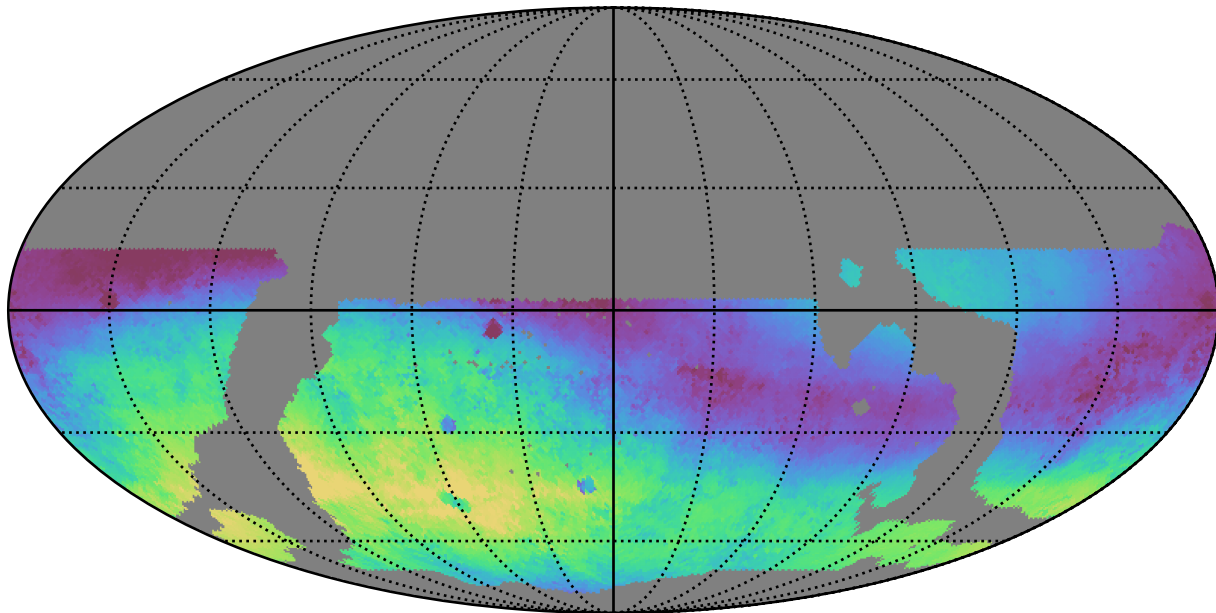
weather_cloudso31v3.4_10yrs WFD g band: Median skyBrightness
