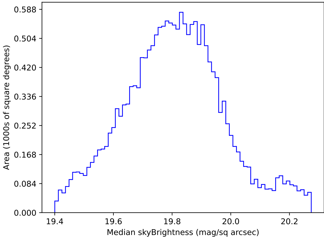
weather_cloudso31v3.4_10yrs WFD all bands: Median skyBrightness
