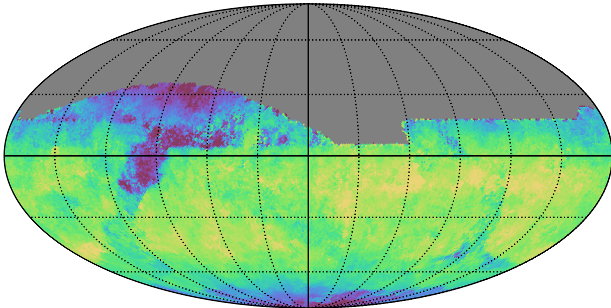
weather_cloudso31v3.4_10yrs All sky z band: Median skyBrightness
