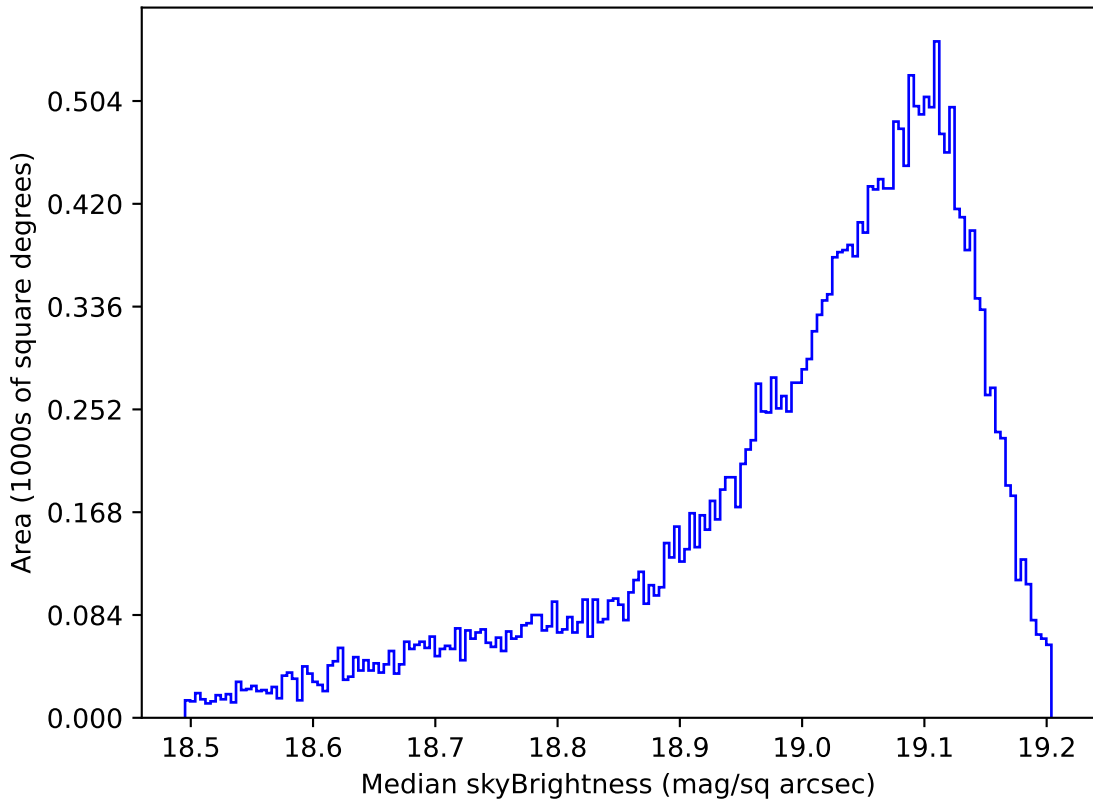
weather_cloudso31v3.4_10yrs All sky z band: Median skyBrightness
