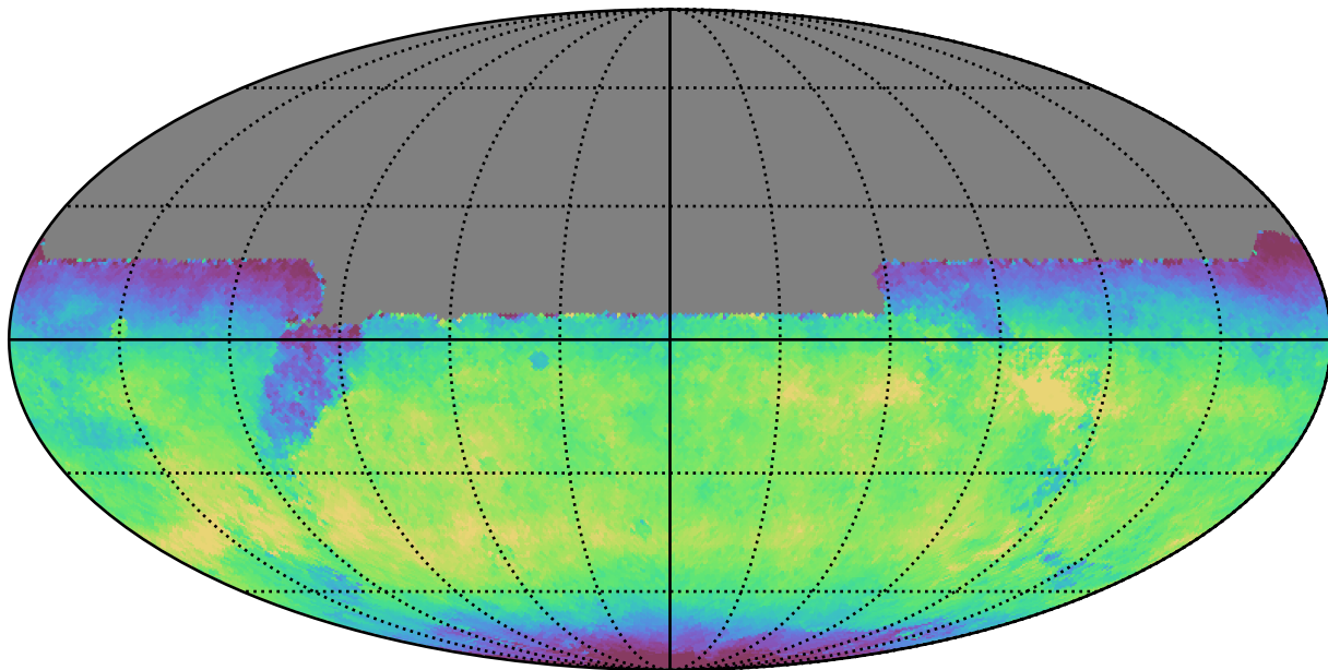
weather_cloudso31v3.4_10yrs All sky y band: Median skyBrightness
