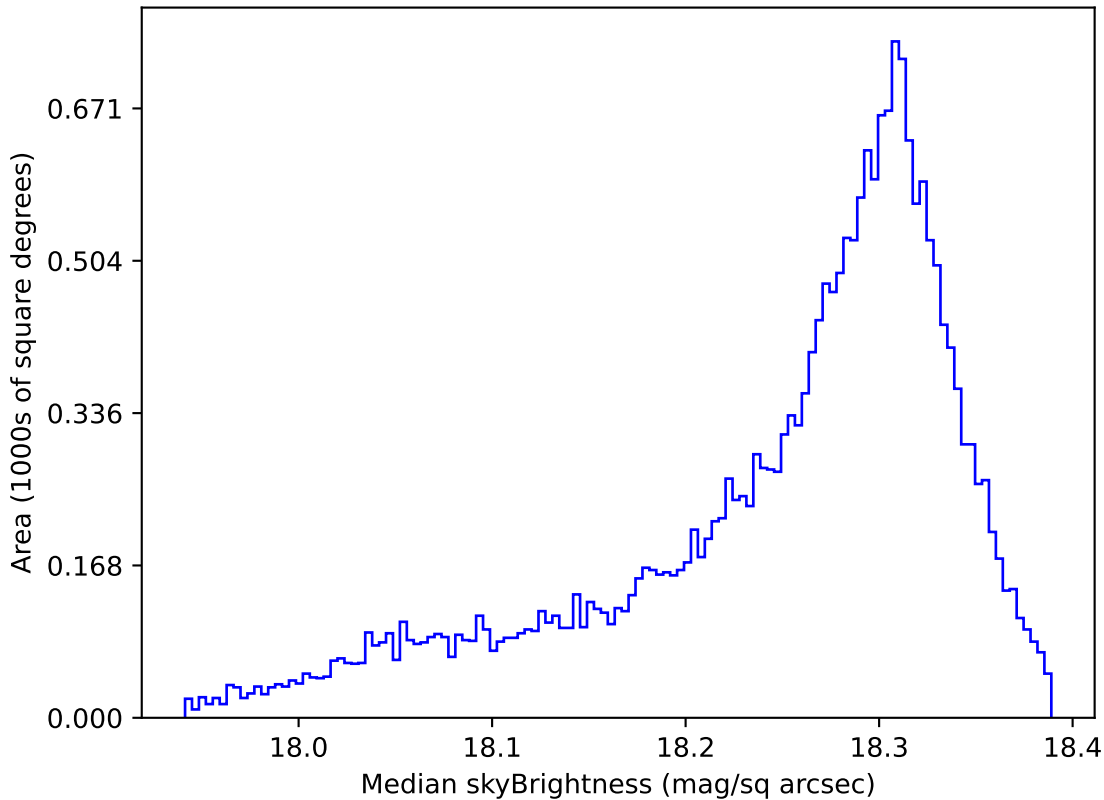
weather_cloudso31v3.4_10yrs All sky y band: Median skyBrightness
