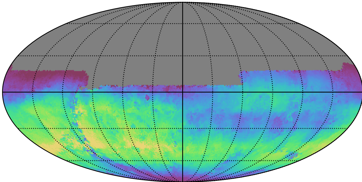
weather_cloudso31v3.4_10yrs All sky u band: Median skyBrightness
