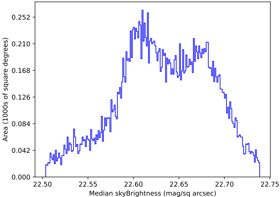
weather_cloudso31v3.4_10yrs All sky u band: Median skyBrightness
