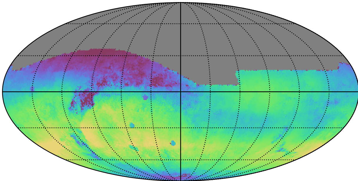
weather_cloudso31v3.4_10yrs All sky r band: Median skyBrightness
