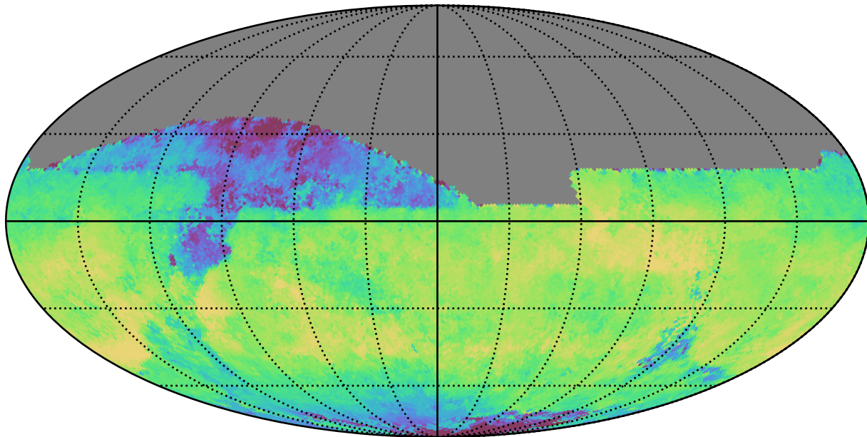
weather_cloudso31v3.4_10yrs All sky i band: Median skyBrightness
