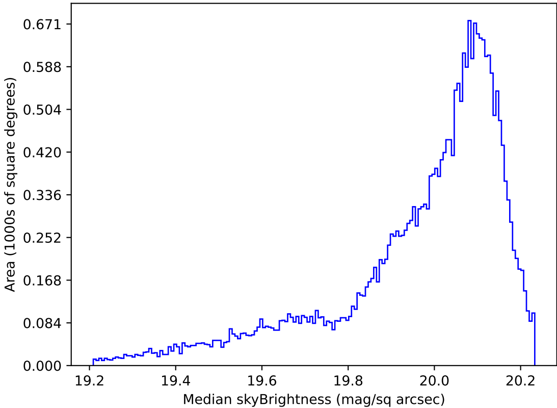
weather_cloudso31v3.4_10yrs All sky i band: Median skyBrightness
