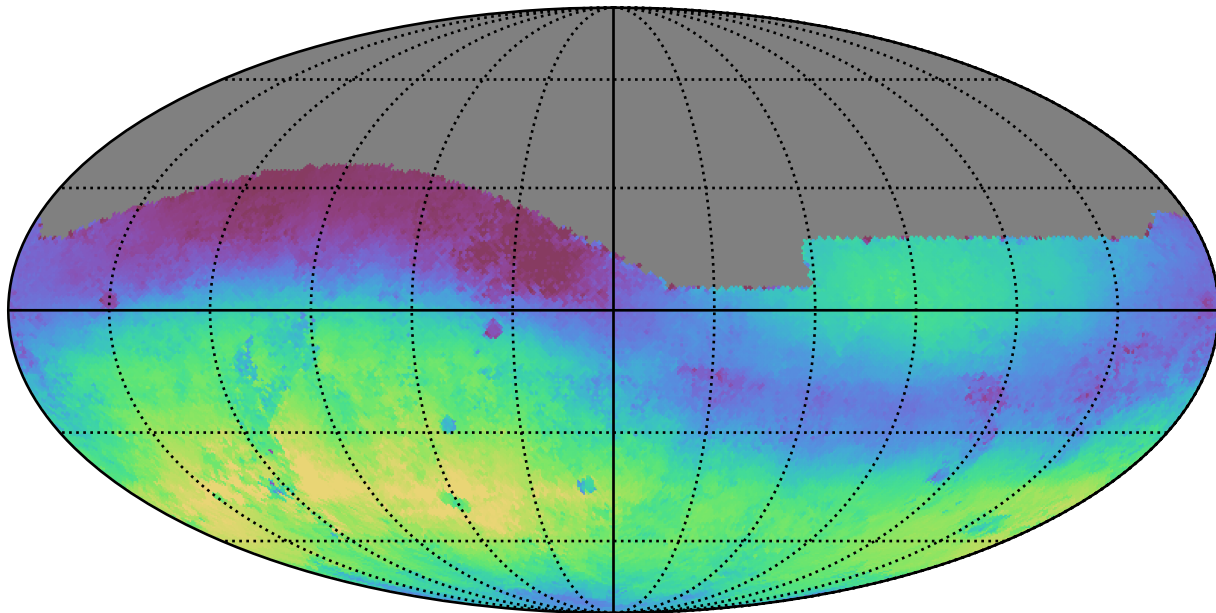
weather_cloudso31v3.4_10yrs All sky g band: Median skyBrightness
