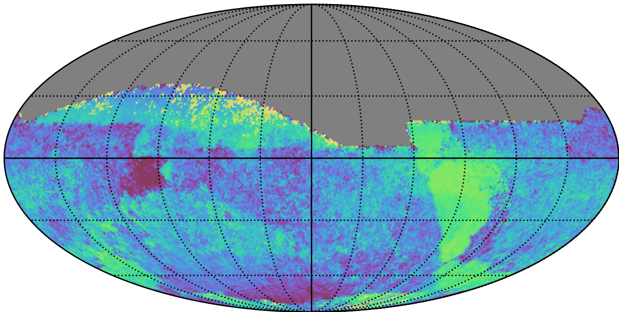
weather_cloudso31v3.4_10yrs All sky all bands: Median skyBrightness
