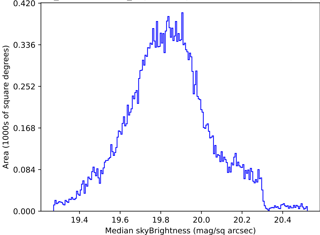
weather_cloudso31v3.4_10yrs All sky all bands: Median skyBrightness
