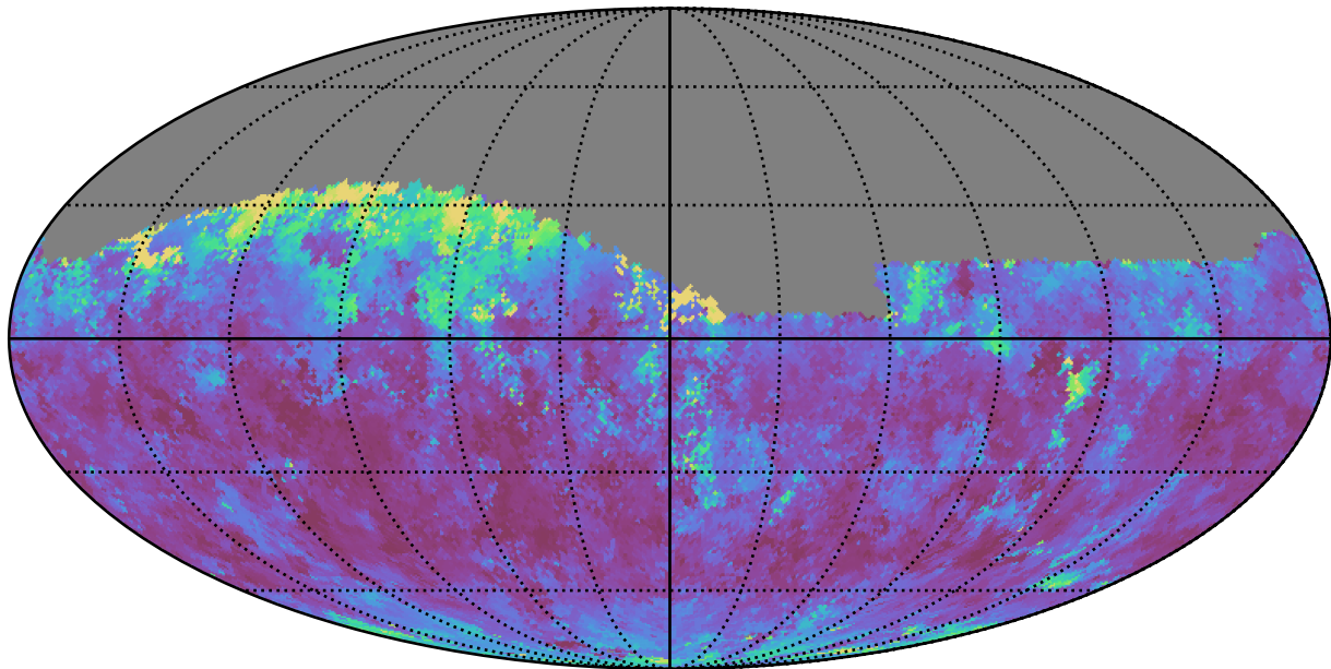
weather_cloudso31v3.4_10yrs Yr 1 z band: Median seeingGeom
