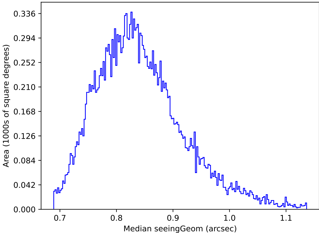
weather_cloudso31v3.4_10yrs Yr 1 y band: Median seeingGeom
