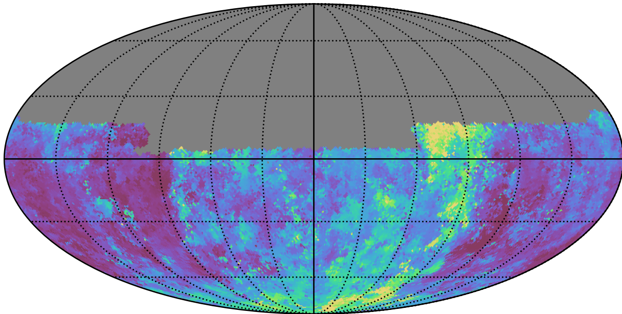
weather_cloudso31v3.4_10yrs Yr 1 u band: Median seeingGeom
