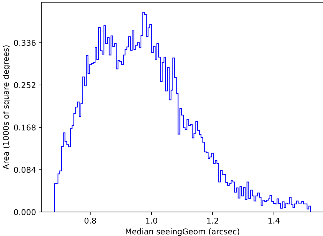
weather_cloudso31v3.4_10yrs Yr 1 u band: Median seeingGeom
