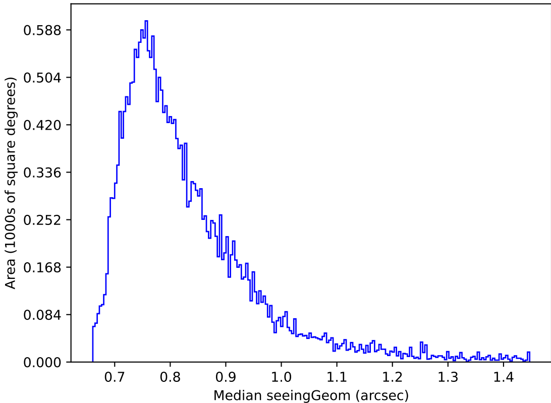
weather_cloudso31v3.4_10yrs Yr 1 i band: Median seeingGeom
