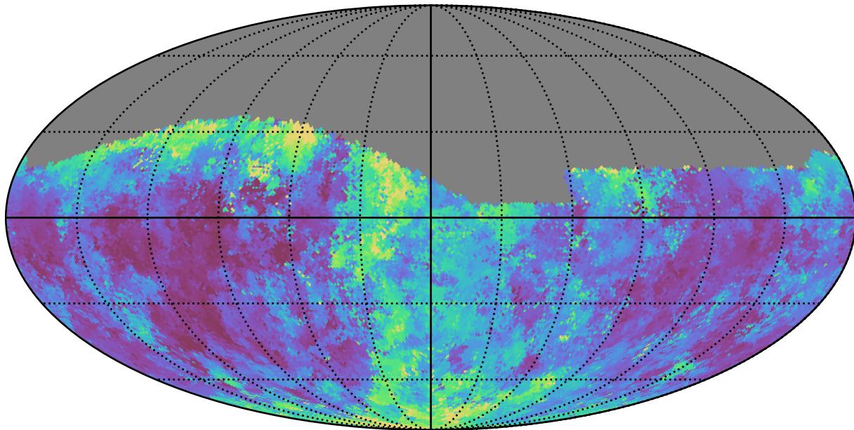
weather_cloudso31v3.4_10yrs Yr 1 g band: Median seeingGeom
