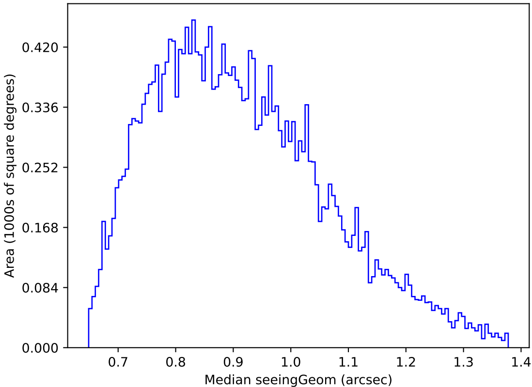
weather_cloudso31v3.4_10yrs Yr 1 g band: Median seeingGeom
