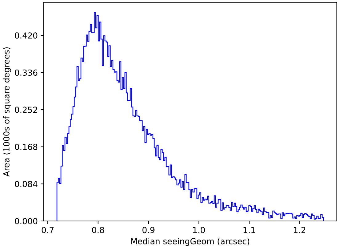
weather_cloudso31v3.4_10yrs Yr 1 all bands: Median seeingGeom
