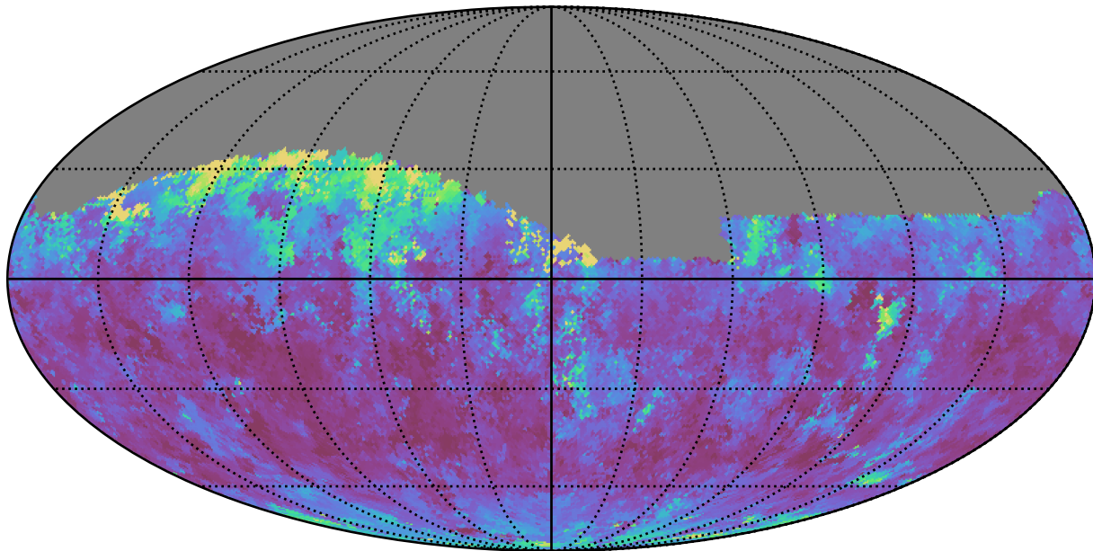
weather_cloudso31v3.4_10yrs Yr 1 z band: Median seeingEff
