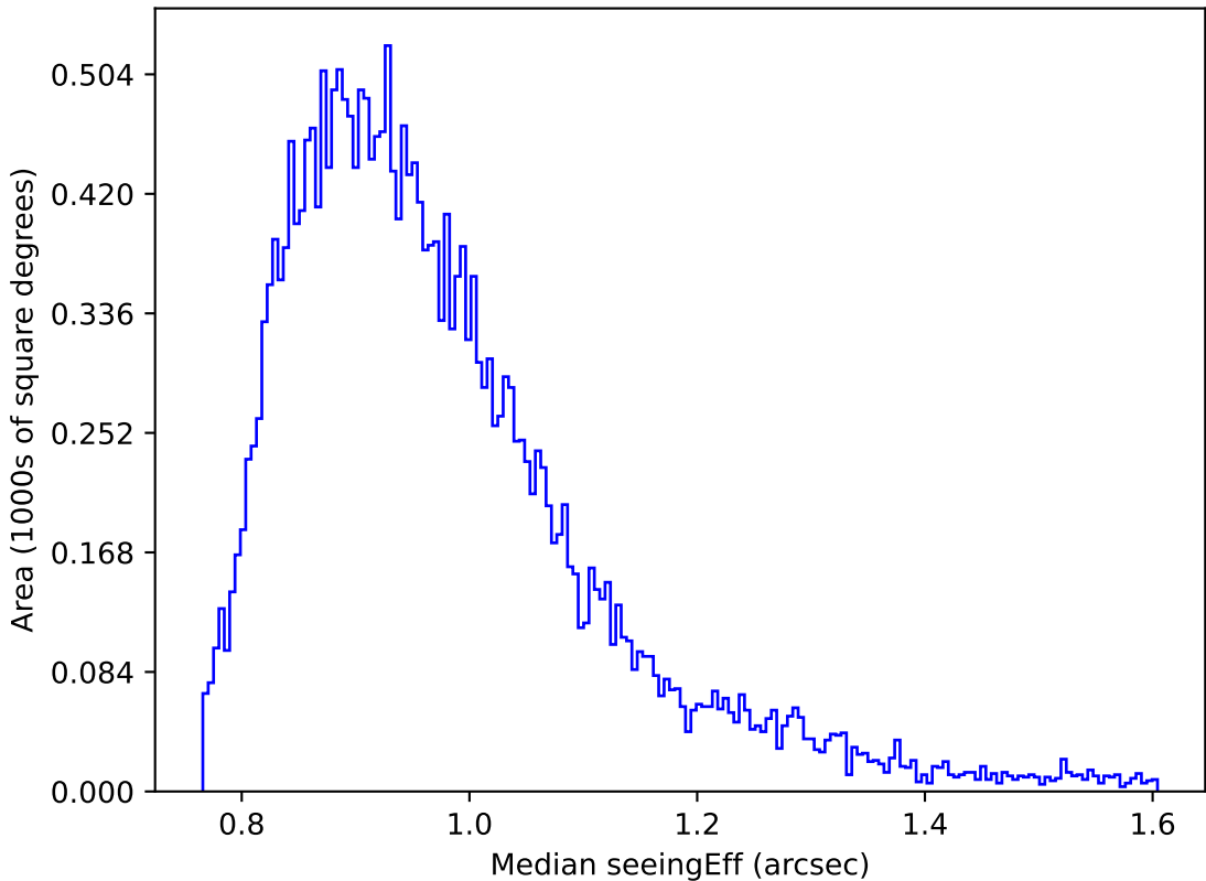
weather_cloudso31v3.4_10yrs Yr 1 z band: Median seeingEff
