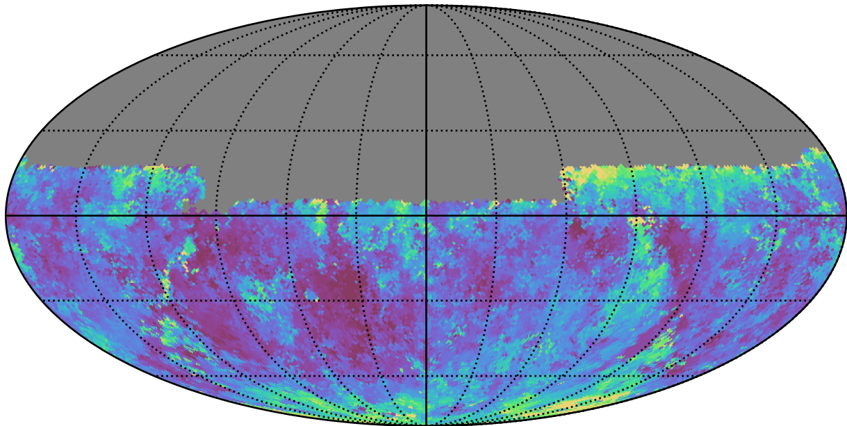
weather_cloudso31v3.4_10yrs Yr 1 y band: Median seeingEff
