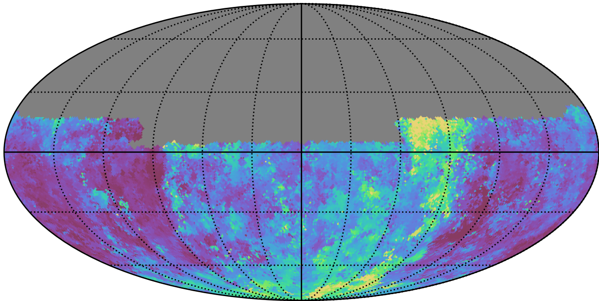
weather_cloudso31v3.4_10yrs Yr 1 u band: Median seeingEff
