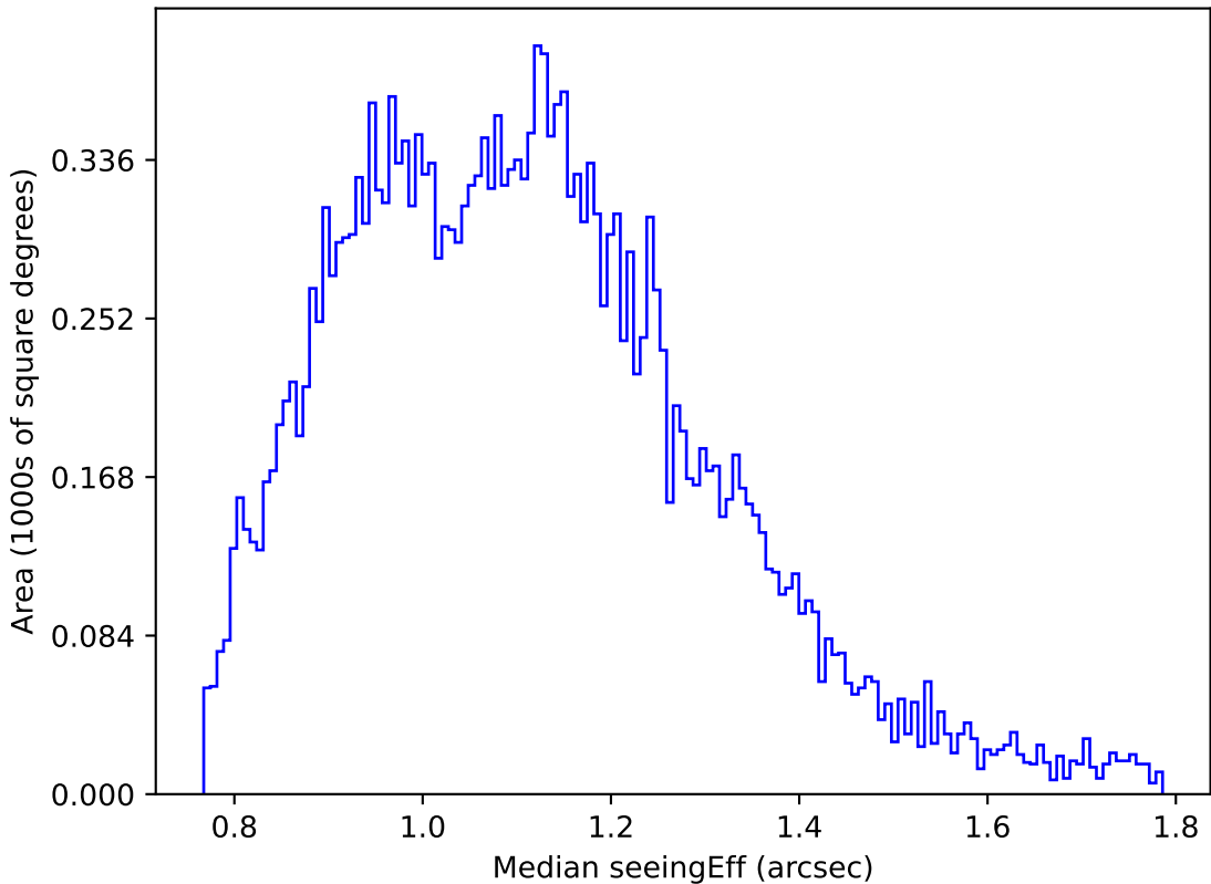
weather_cloudso31v3.4_10yrs Yr 1 u band: Median seeingEff
