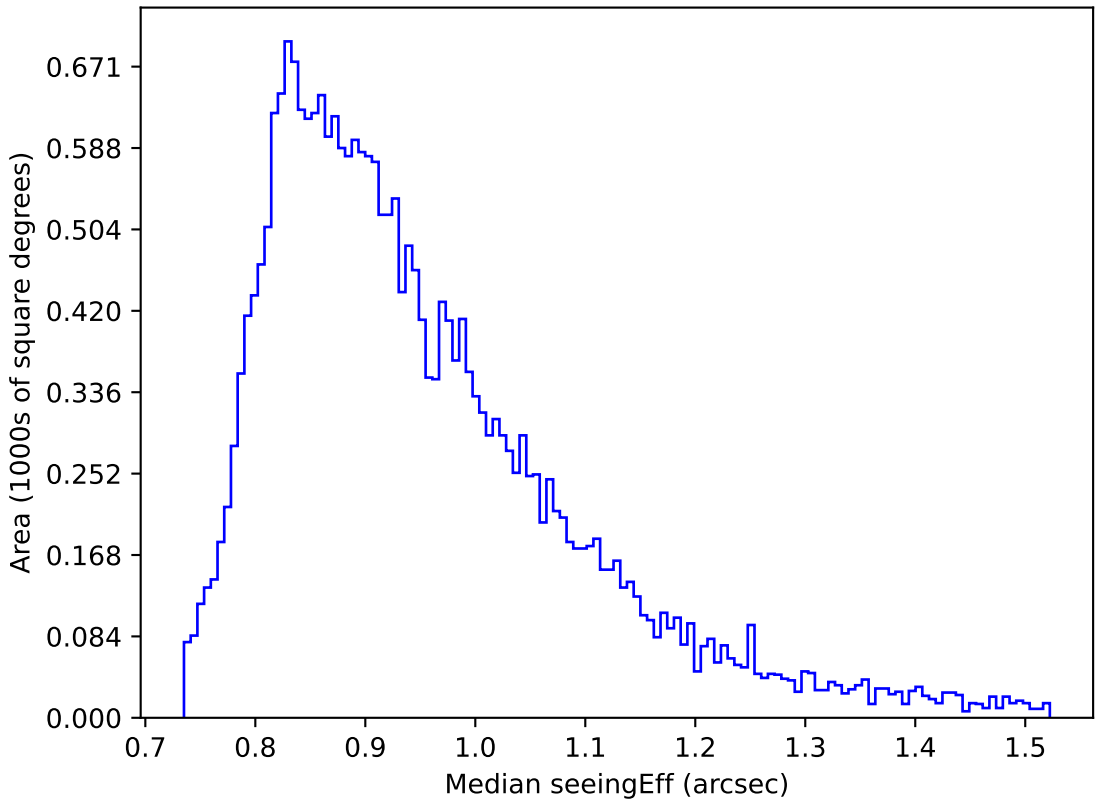
weather_cloudso31v3.4_10yrs Yr 1 r band: Median seeingEff
