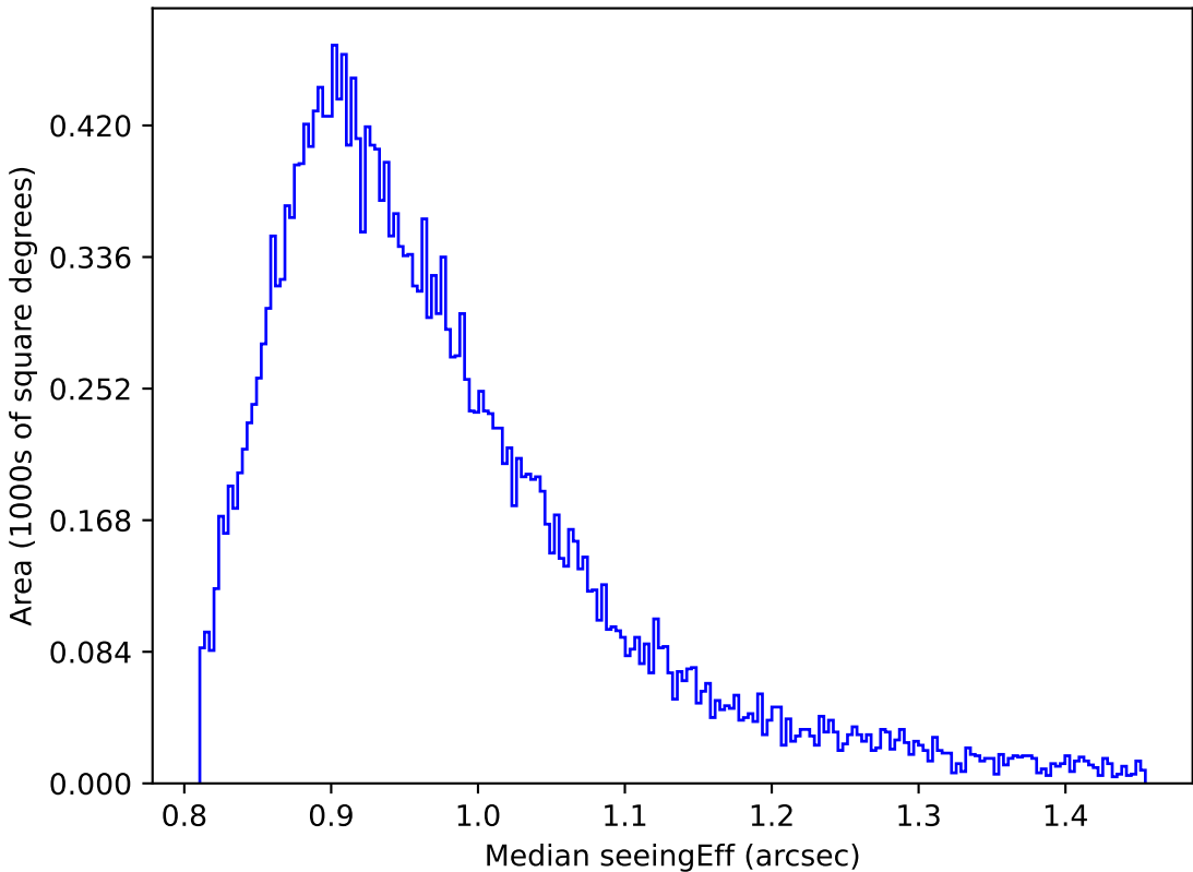
weather_cloudso31v3.4_10yrs Yr 1 all bands: Median seeingEff
