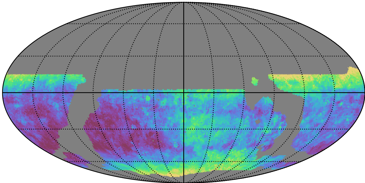
weather_cloudso31v3.4_10yrs WFD z band: Median seeingEff
