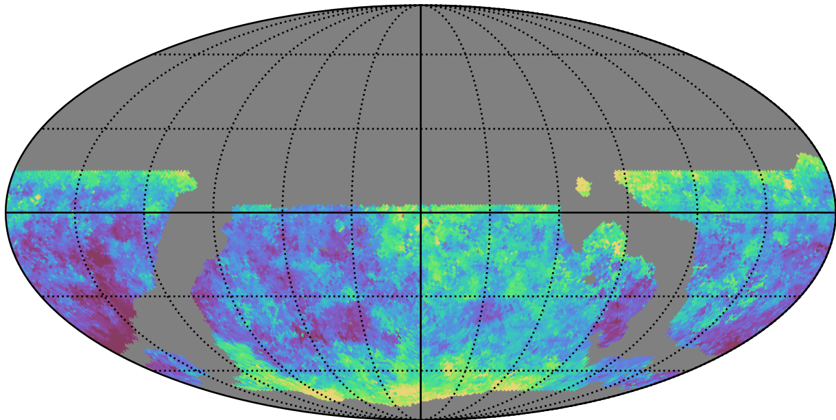
weather_cloudso31v3.4_10yrs WFD u band: Median seeingEff
