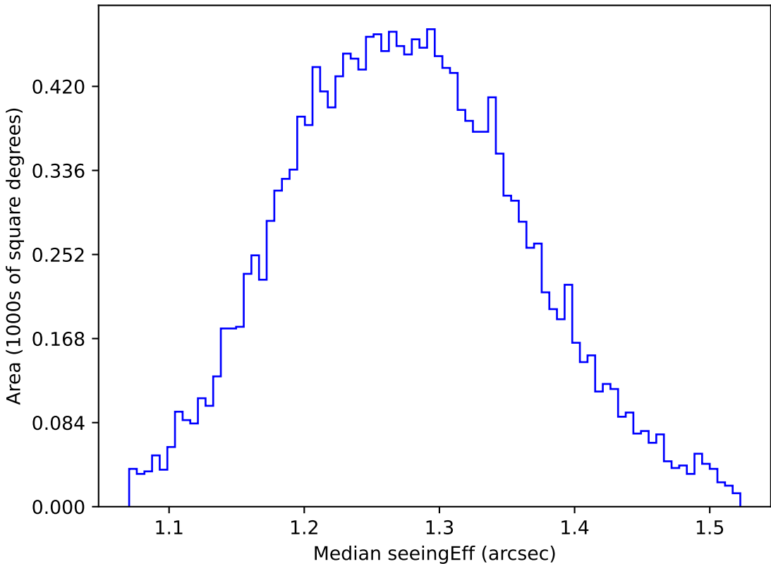
weather_cloudso31v3.4_10yrs WFD u band: Median seeingEff
