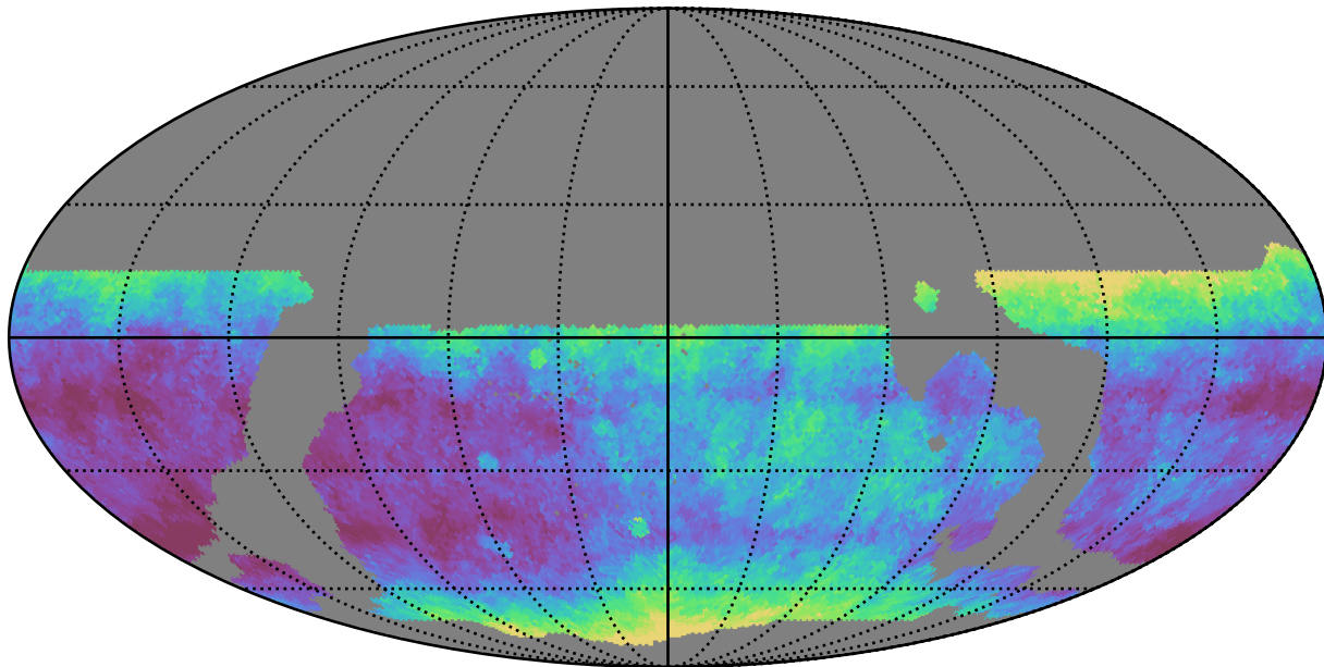
weather_cloudso31v3.4_10yrs WFD r band: Median seeingEff
