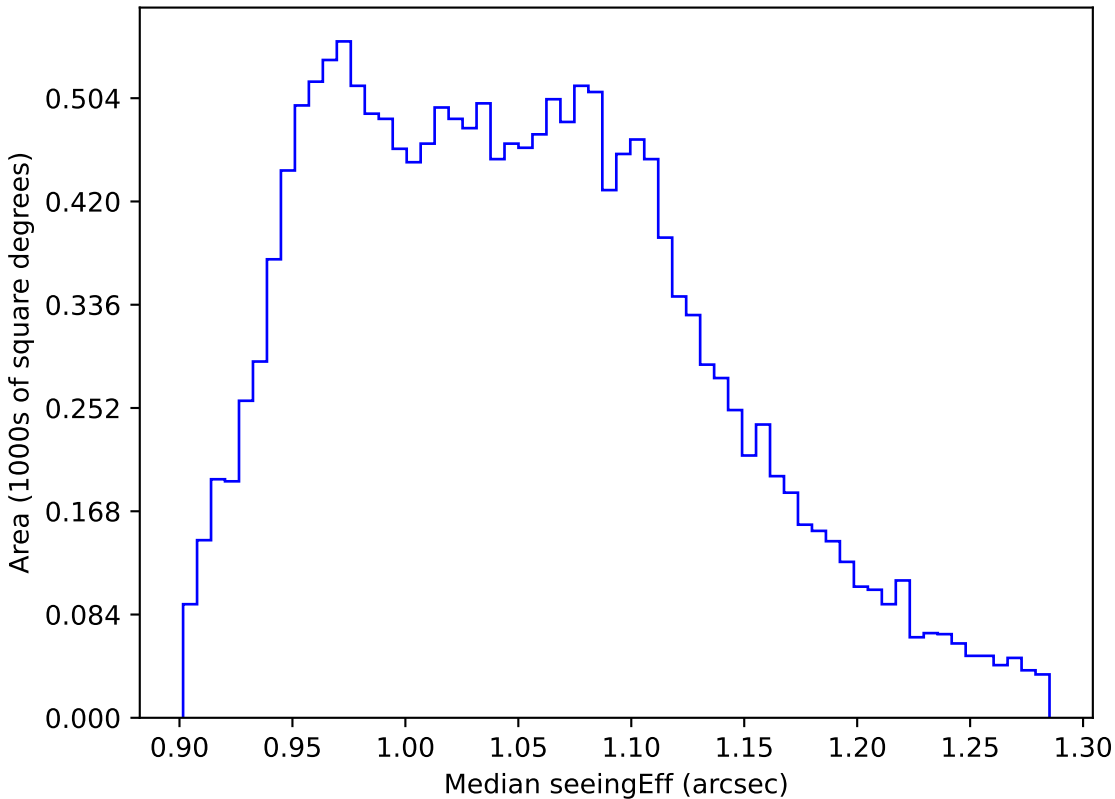
weather_cloudso31v3.4_10yrs WFD r band: Median seeingEff
