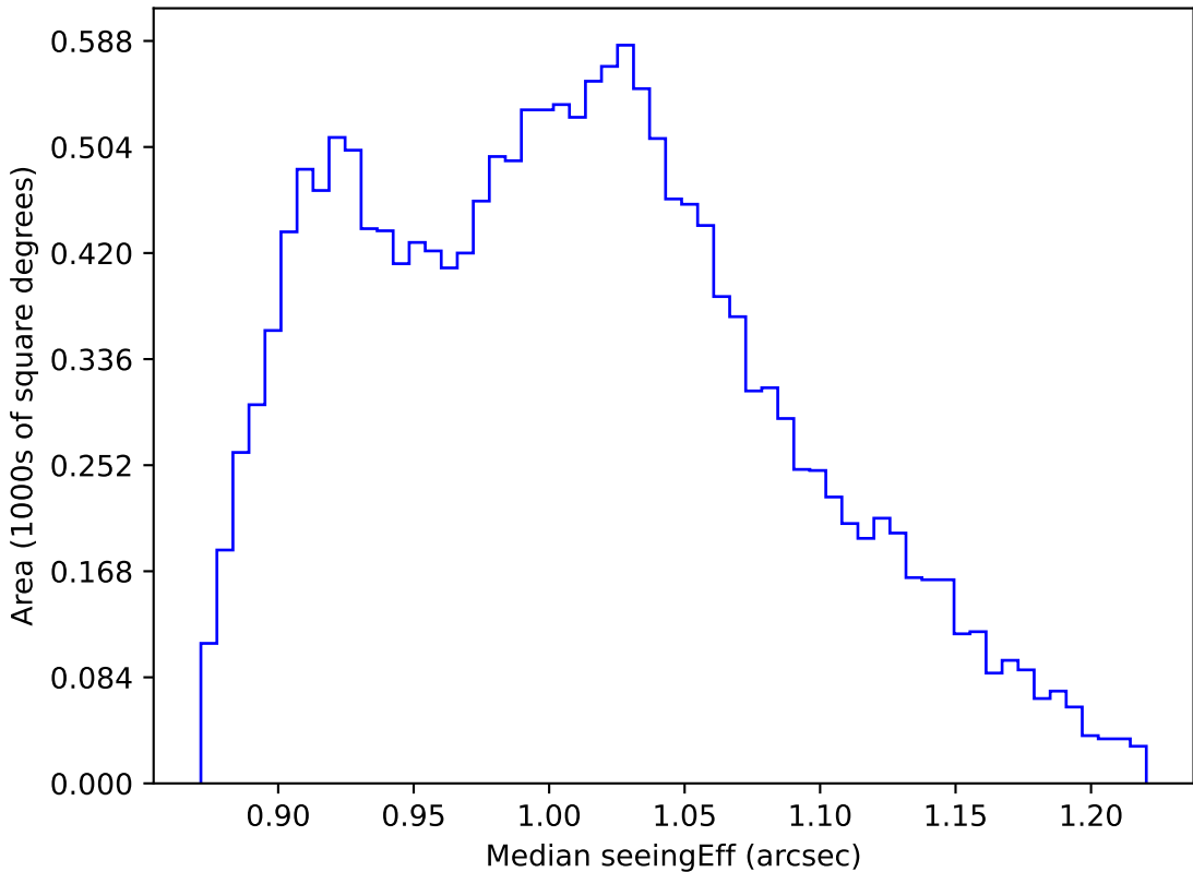
weather_cloudso31v3.4_10yrs WFD i band: Median seeingEff
