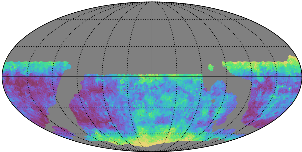
weather_cloudso31v3.4_10yrs WFD g band: Median seeingEff
