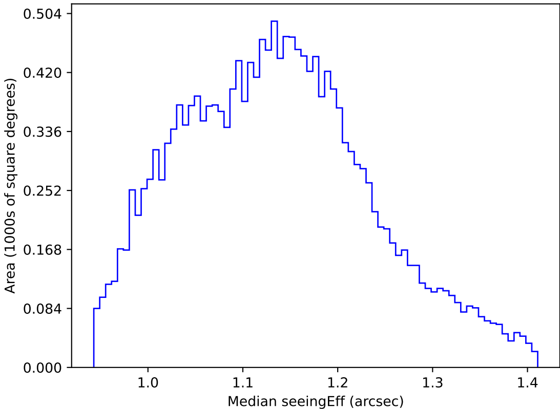
weather_cloudso31v3.4_10yrs WFD g band: Median seeingEff
