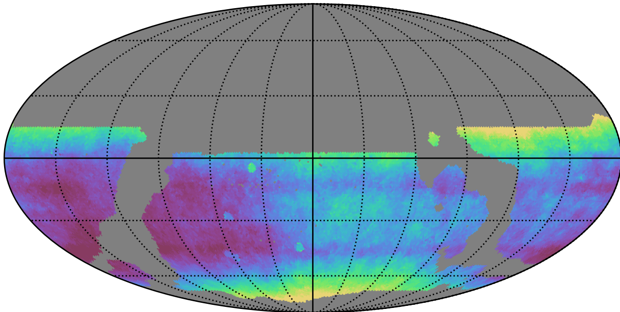
weather_cloudso31v3.4_10yrs WFD all bands: Median seeingEff
