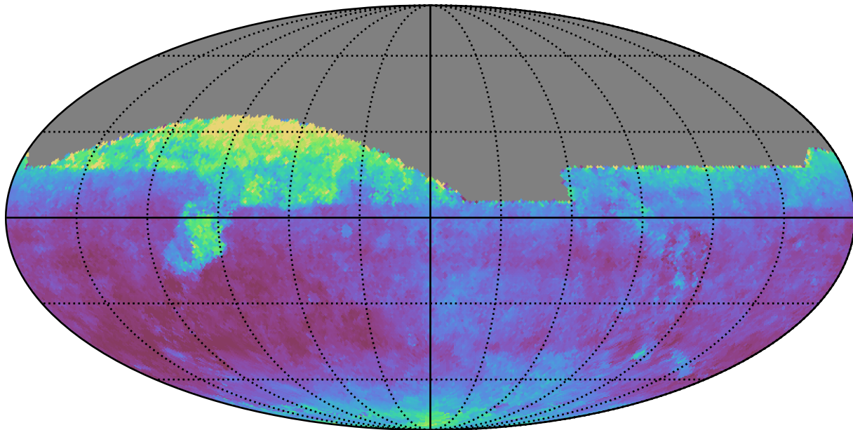
weather_cloudso31v3.4_10yrs All sky z band: Median seeingEff
