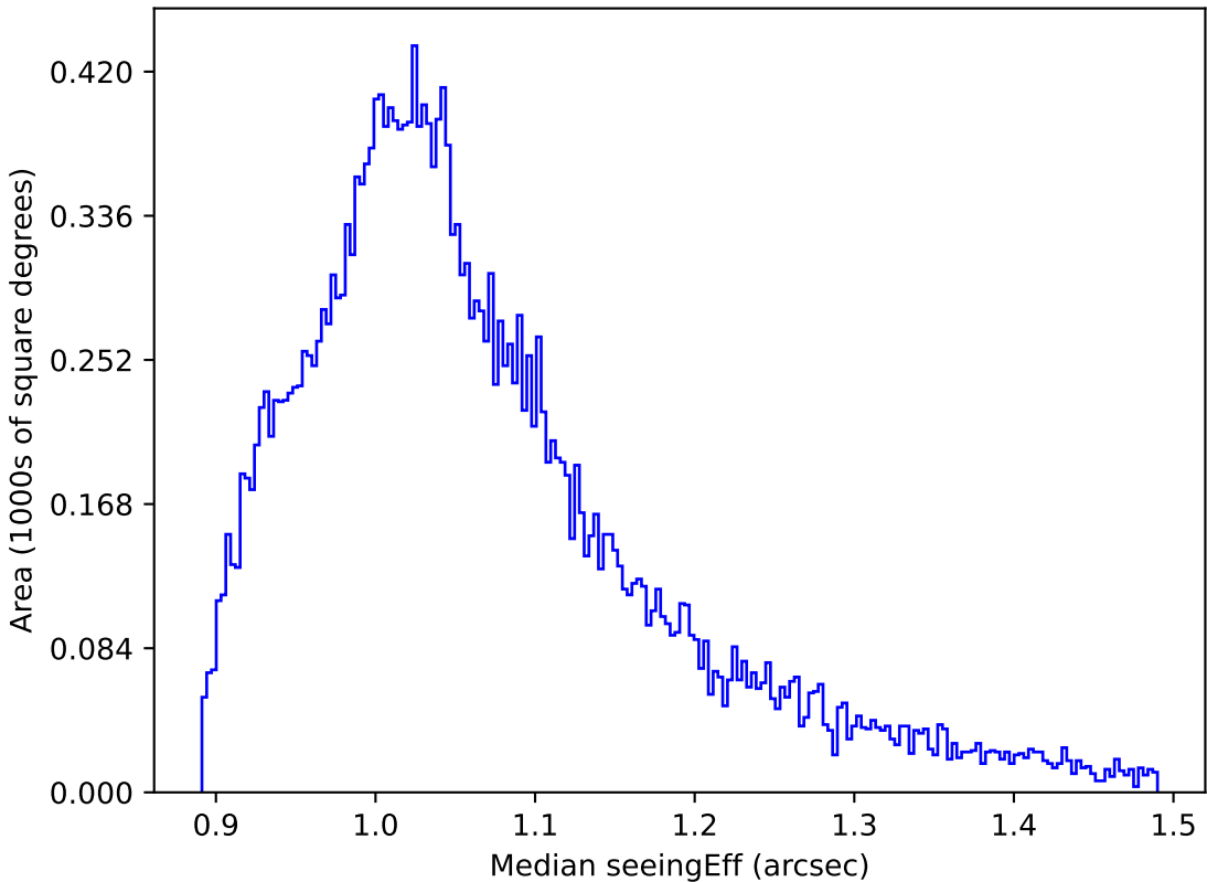
weather_cloudso31v3.4_10yrs All sky z band: Median seeingEff
