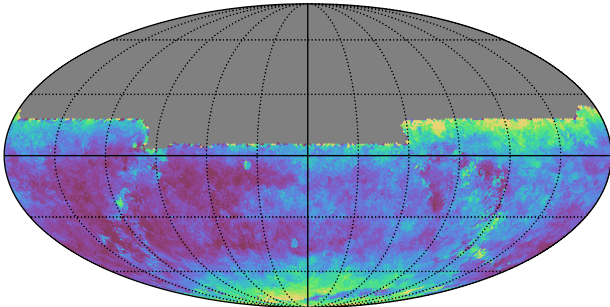
weather_cloudso31v3.4_10yrs All sky y band: Median seeingEff
